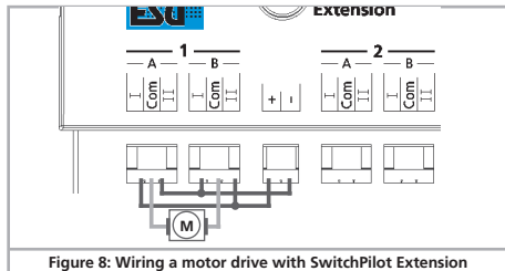
Figure 8: Wiring a motor drive with SwitchPilot Extension
