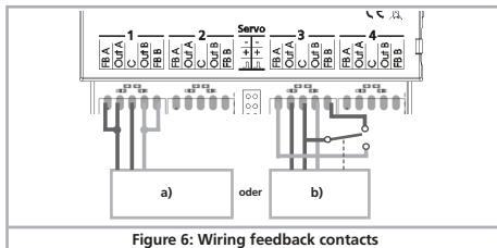
Figure 6: Wiring feedback contacts
