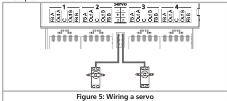
Figure 5: Wiring a servo
