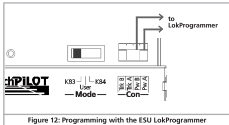
Figure 12: Programming with the ESU LokProgrammer
