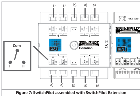
Figure 7: SwitchPilot assembled with SwitchPilot Extension
