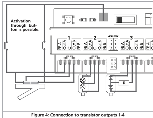
Figure 4: Connection to transistor outputs 1-4
