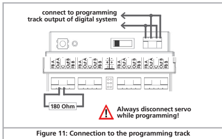
Figure 11: Connection to the programming track
