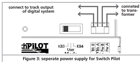
Figure 3: separate power supply for Switch Pilot
